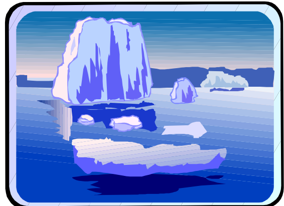
iceberg
