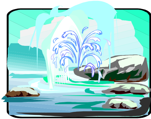
Geyser
